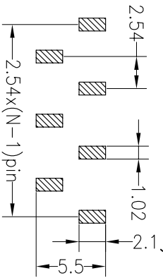
Recommended P.C.B. Layout (Top Side) (PCB BOARD TOLERANCE ±0.05)
